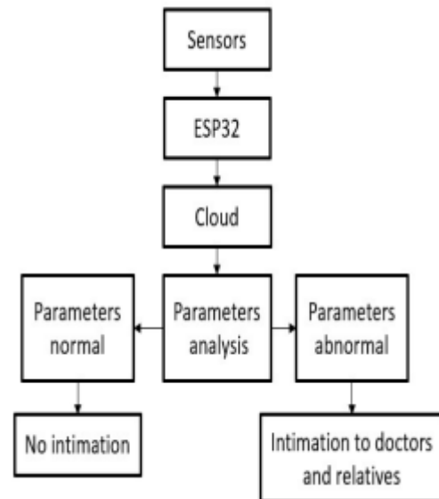
Figure 3: Diagram of smart healthcare system [21]
