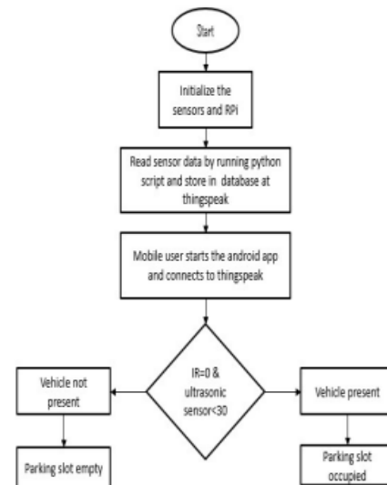
Figure 2: Diagram of smart parking system [19]
