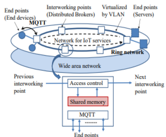
Fig. 3. Architecture of the proposed scheme for distributed brokers.
