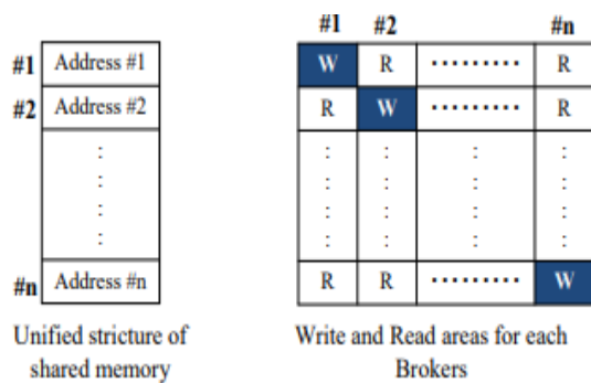
Fig. 7. The structure of the shared memory.
