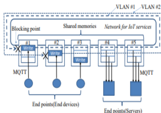
Fig. 4. Communication among shared memory in distributed brokers.
