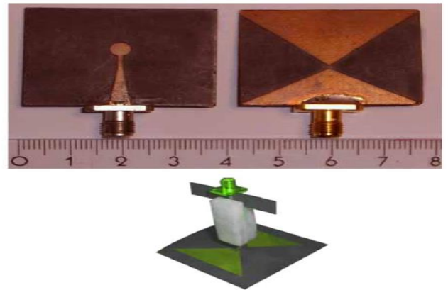
Fig. 9. (Left) Aperture coupled bowtie antenna; bottom view with feed line. (Right) Top view; symmetric fed bowtie antenna with balloon.
