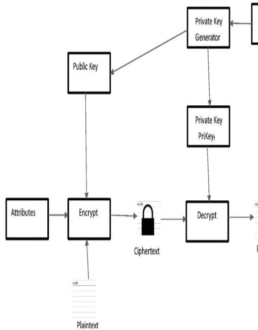
Fig. 1. Key Policy Attribute Based Encryption from Lattices.
