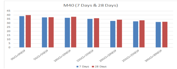
Graph 6.3 – 7&28 Days strength of different proportions of M40 grade concrete
