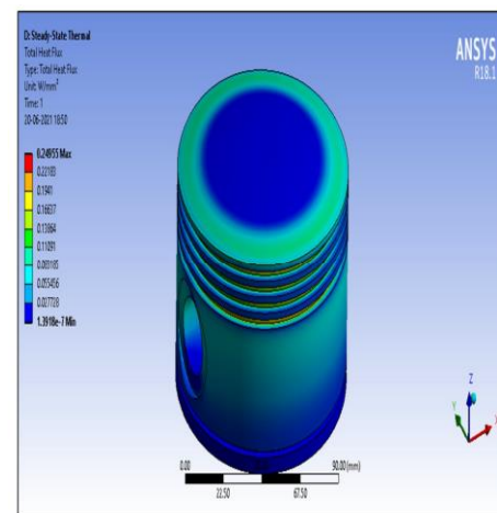
Figure 4.3 heat flux
