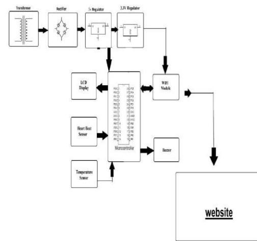
Fig 2 block digram
