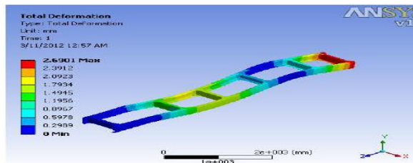
Deformation of modified chassis
