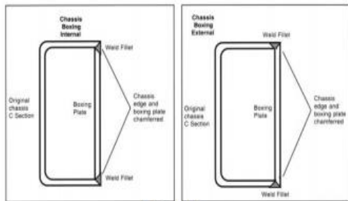
Fig 1 Boxing
