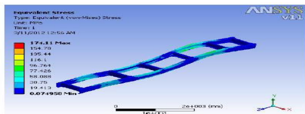
Equivalent stress in chassis frame
