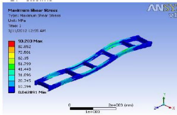
Maximum shear stress in chassis frame
