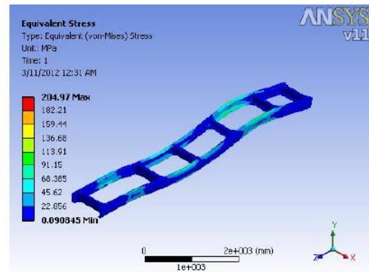
Equivalent stress in chassis frame
