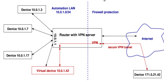
Fig. 2 VPN – virtual private network
