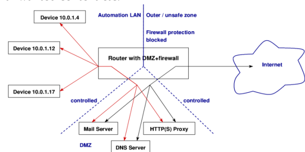
Fig. 3 DMZ – demilitarised (network) zone
