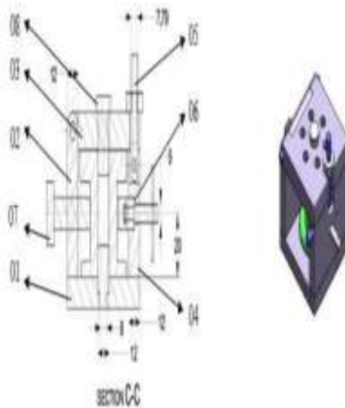
Fig.3 Assembly design of Drill Jig
