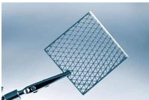
Fig 8: Metamaterial Slab
