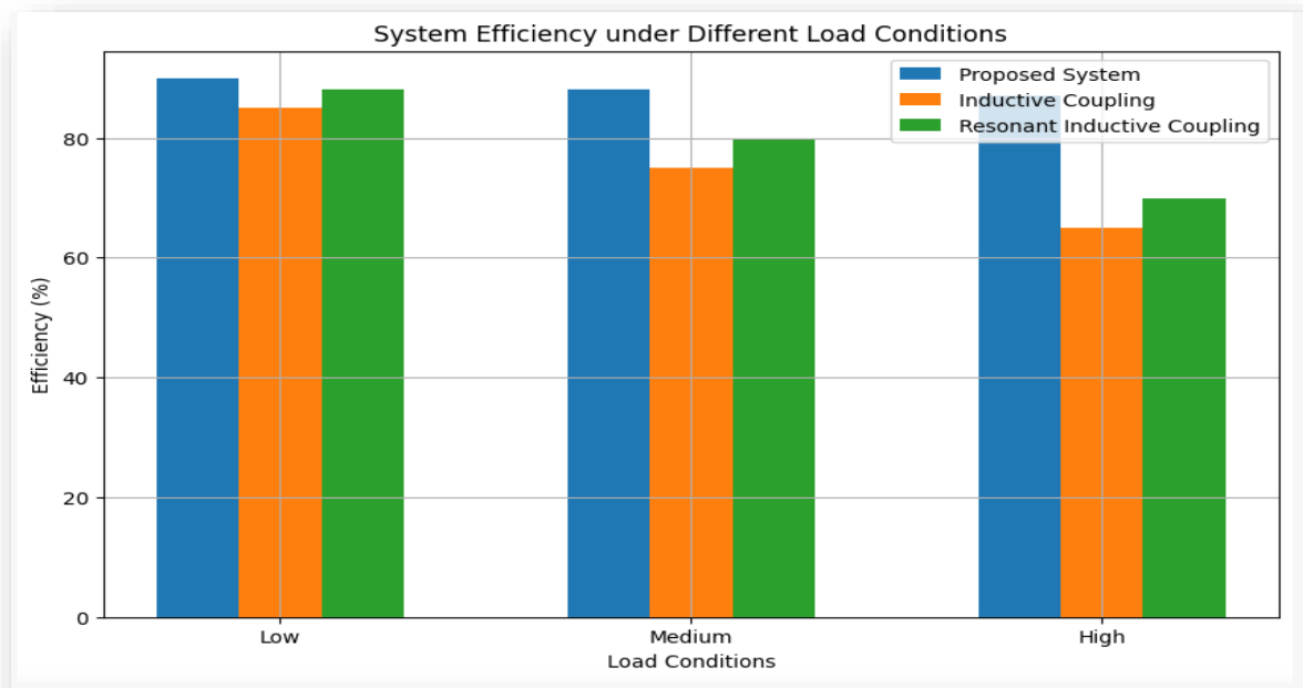
Fig 18: A Bar Chart Showing Efficiency at Different Load Conditions
