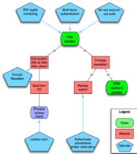
Fig. 2. Attack Tree
